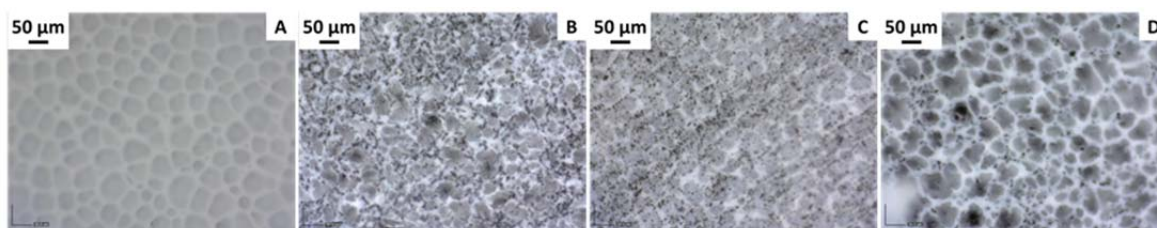
Figure 3: Digital microscope images of the MPLs surface: A) no filler, B) 0.9% Ketjen Black; C) 0.9% HSAG 300 and D) 0.9% carbon nanotubes.
