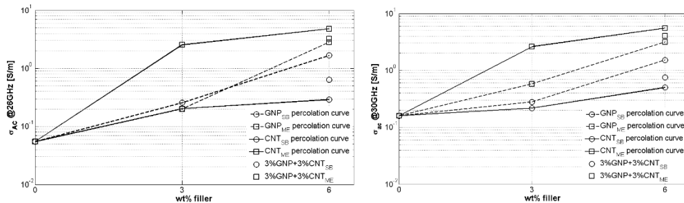
Figure 5: AC electrical conductivity, at fixed frequency of 26 GHz (left) and 30 GHz (right), vs filler amount.
