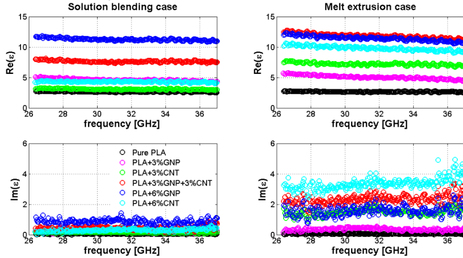
Figure 3: Re and Im part of the complex permittivity for SB (left) and ME (right) nanocomposites filaments compared with pure PLA
