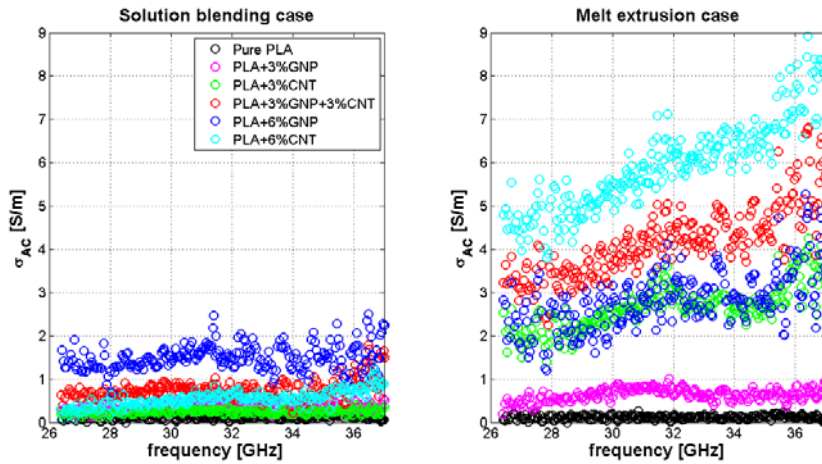
Figure 4: AC electrical conductivity for SB (left) and ME (right) filament samples compared with pure PLA
