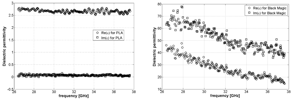
Figure 2: Results for neat PLA (left) and BM (right)
