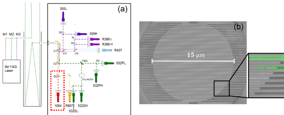
Figure 1: (a) Scheme of MALIA Lidar system. M1, M2, M3 represent the laser wavelengths emitted in the atmosphere ( 1064 \text{ nm} , 532 \text{ nm} , 355 \text{ nm} ). D1, D2, D3, D4 are the dichroic mirrors used to separate the different wavelengths. BS and PBS are the beamsplitters adopted to divide the signal and the polarizations. The red box highlights the channel used in the present work. (b) A SEM image of NbTiN SNSPD.
