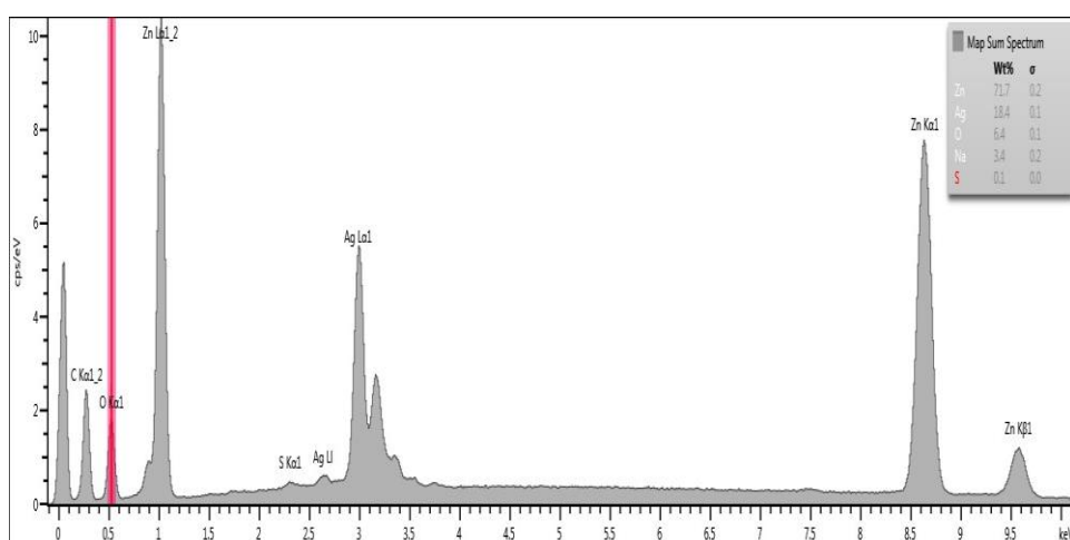
Figure 3: EDX spectra of ternary Ag/Ag 2 S/ZnO nanopowder.
