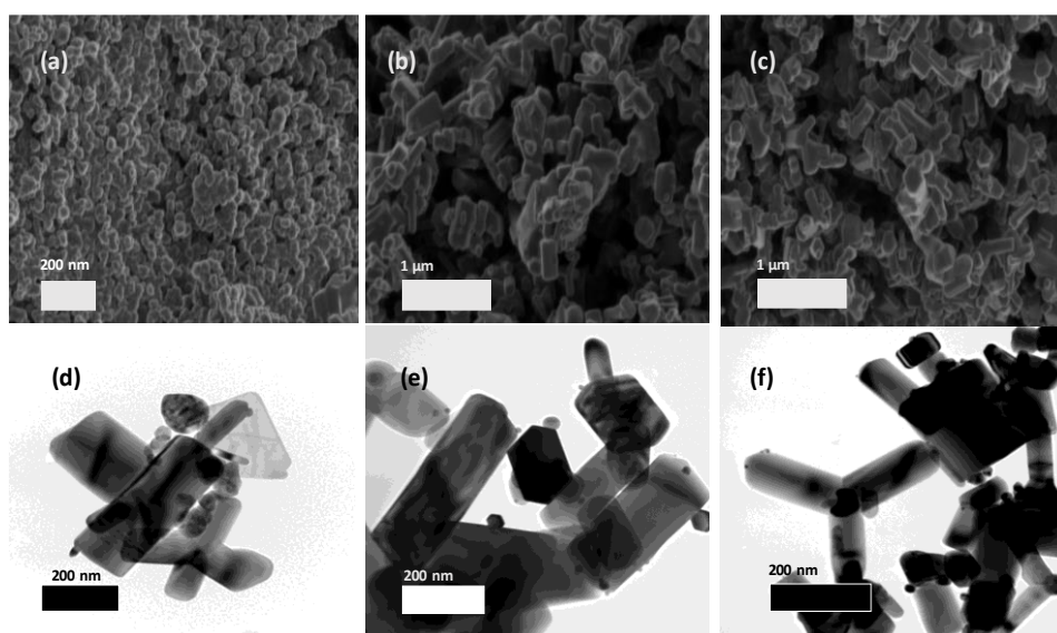
Figure 2: SEM (a), (b), (c) and TEM (d), (e), (f) images of ZnO, Ag 2 S/ZnO and Ag/Ag 2 S/ZnO
