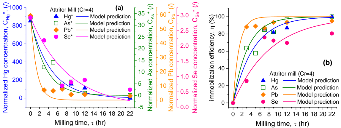
Figure 2. Time evolution of normalized HM concentrations (a) and immobilization efficiency (b) using the Attritor
