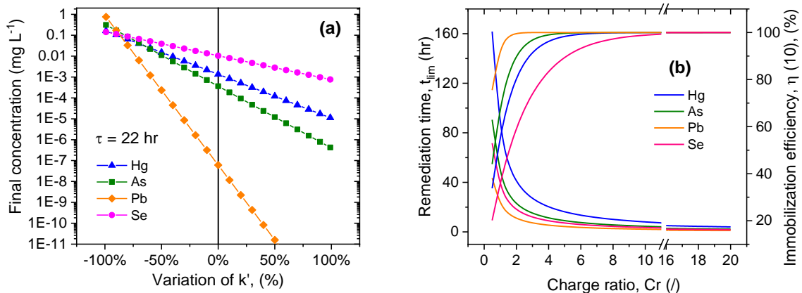
Figure 3. Sensitivity of simulated HMs concentrations in the leachate after 22 hours milling to the variation of the parameter k' (a); simulated effect of Cr change on the remediation time and immobilization efficiency after 10 hours of mechanical treatment (b).
