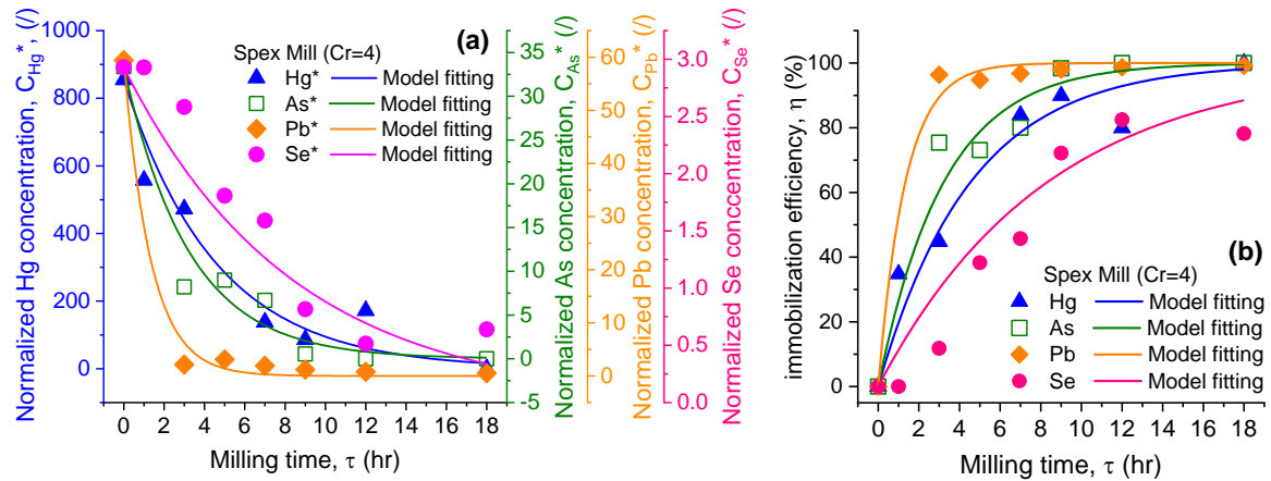
Figure 1. Time evolution of normalized HM concentrations (a) and immobilization efficiency (b) using the SPEX
