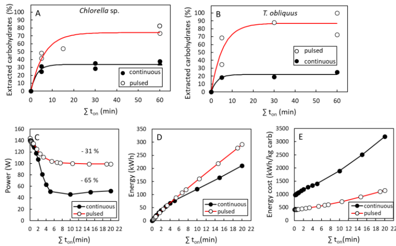
Figure 4. A-B) Extracted carbohydrates as function of time for pulsed and continuous ultrasonication. With solid lines, the fittings obtained with the first order model are shown. C) Applied power. D) Registered drop in applied energy. E) Specific energetic cost for carbohydrate extraction. Amplitude: 90 \mu\text{m} ; biomass: 6 g L -1 .
