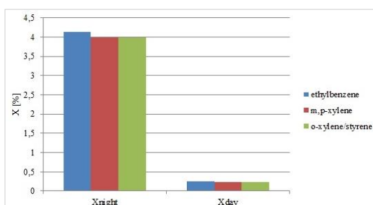
Figure 3 - Night and day removal efficiencies for ethylbenzene, m,p-xylene and o-xylene/styrene obtained by virtually introducing 40 specimens of Zamioculcas zamiifolia ( A_{l,TOT} \approx 23 m 2 ) into the copy shop.
