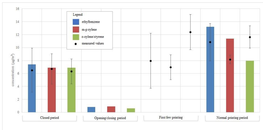
Figure 2: Concentrations values ( \mu\text{g}/\text{m}^3 ) of ethylbenzene, m,p-xylene and o-xylene/styrene calculated and measured with relative uncertainty range (Betha et al., 2011).
