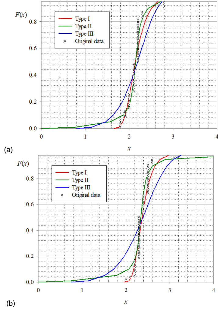
Figure 1: Cumulative distribution curves for (a) 2010 and (b) 2017.
