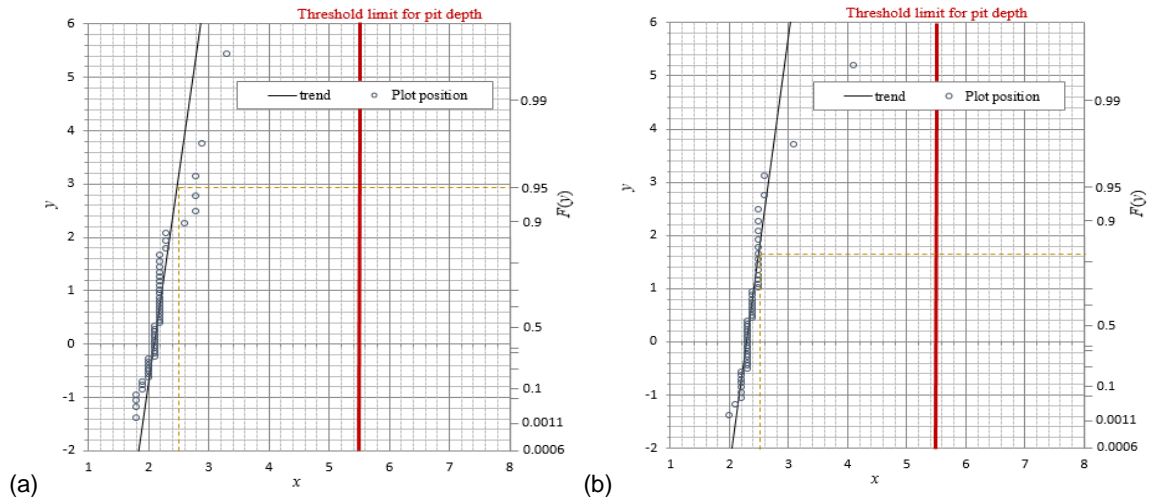
Figure 2: (a) Plot position 2010, (b) Plot position 2017.
