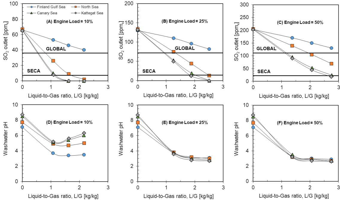
Figure 2: Experimental results of SO 2 outlet emission from scrubber (A,B,C) and wash water pH (D,E,F) as a function of the liquid-to-gas mass ratio ( L/G ) and parametric with four different seawater solutions (Finland Gulf Sea, North Sea, Canary Sea and Kattegat Sea) and three different engine loads (10, 25 and 50%). The lines in Fig. 2A-C denote the maximum allowed SO 2 emissions in SECAs and open sea (GLOBAL)
