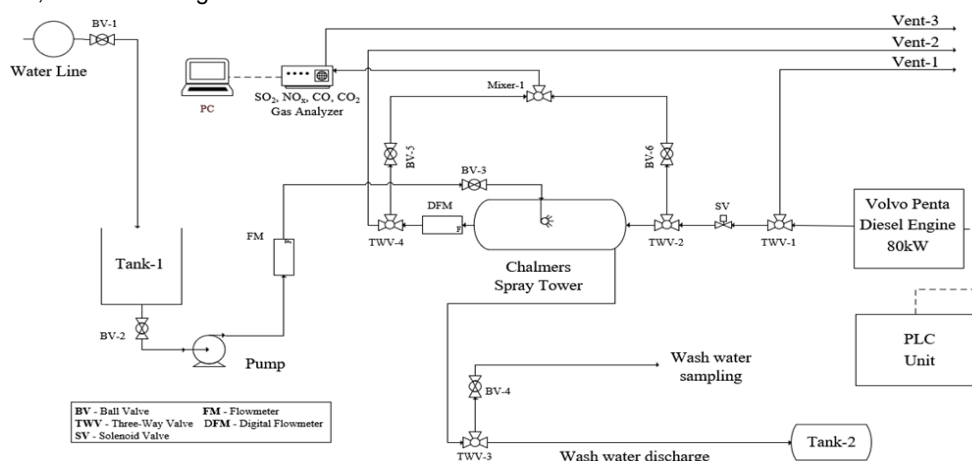
Figure 1: Flowsheet of the experimental pilot-plant
