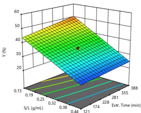
Figure 3: 3d plot showing the effect of solid to liquid ratio (g/mL) and extraction time (min) on the extraction yield.
