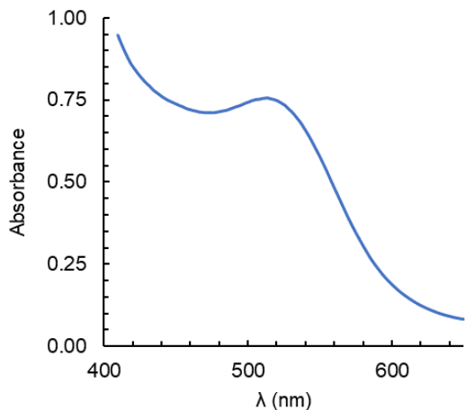
Figure 1: UV-Vis spectrum of the extract obtained employing choline-chloride
