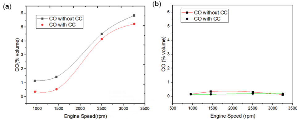
Figure 2: CO emission as a function of speed for (a) gasoline and (b) LPG engine
