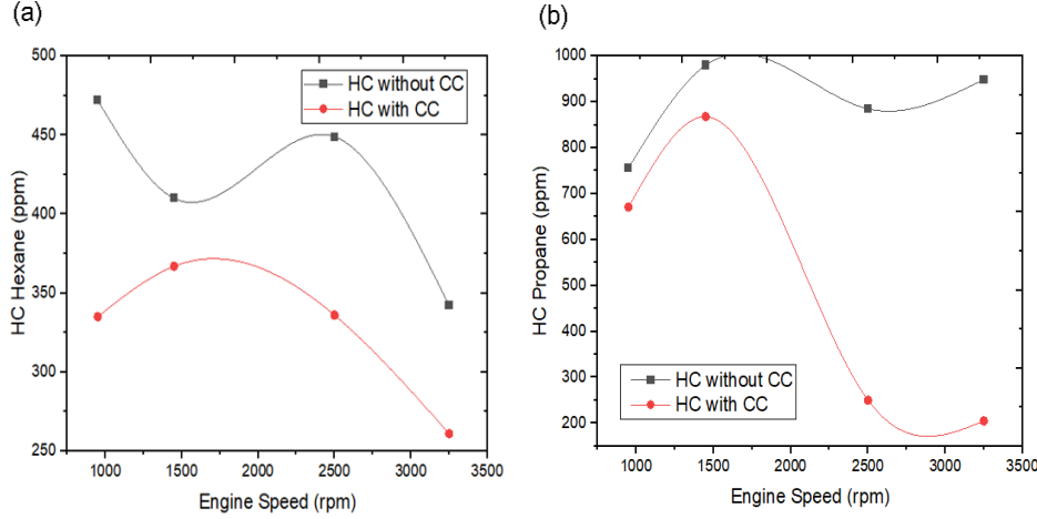
Figure 3: HC emission as a function of speed for (a) petrol engine and (b) LPG
