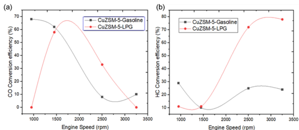
Figure 4: (a) CO reduction as a function of speed and (b) HC reduction as a function of speed
