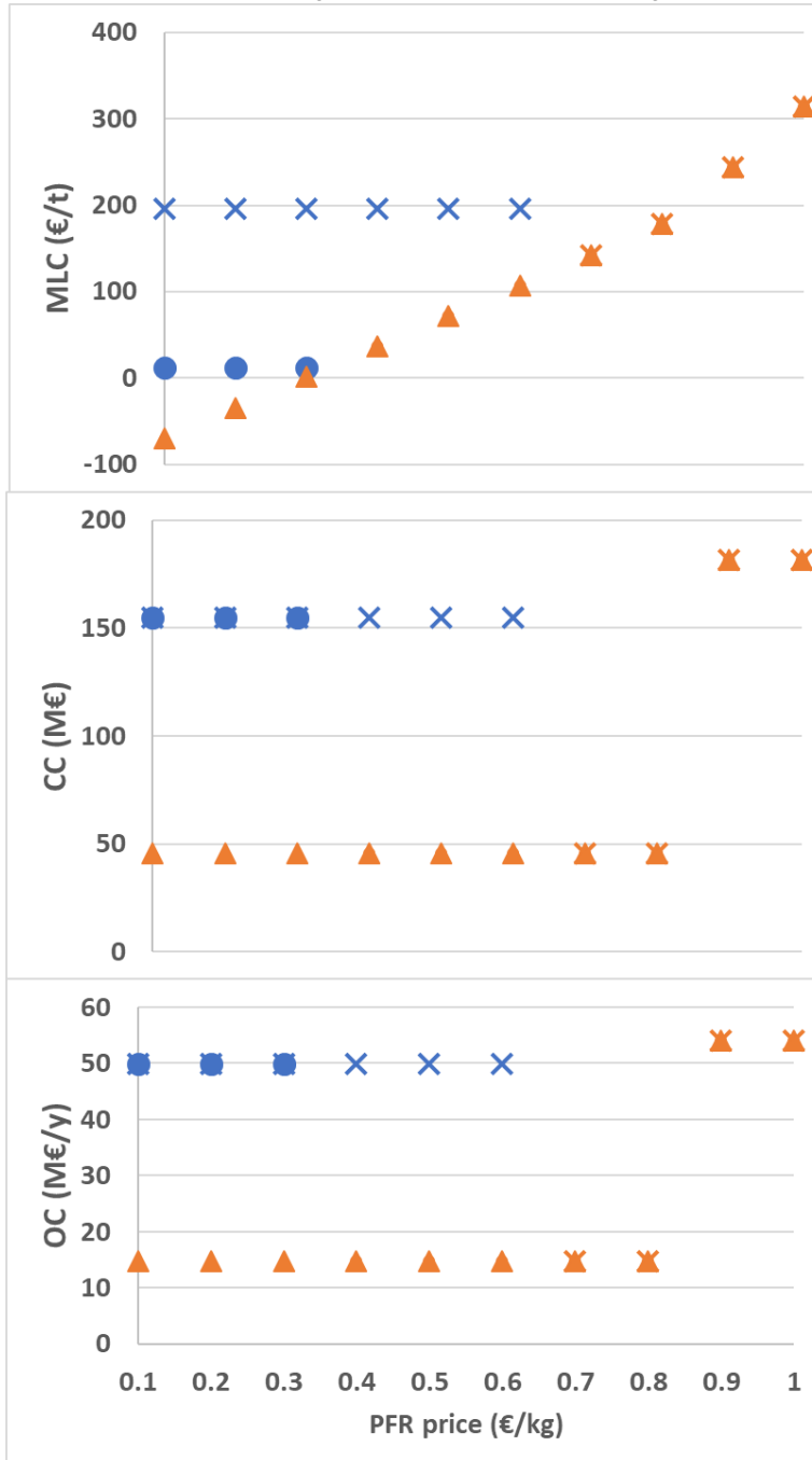
Figure 2: Maximum Lignin Cost (MLC), capital costs (CC), operating costs (OC) as a function of the PFR and parametric in the AM selling price: ▲ 0.60 €/kg; ● 1.20 €/kg; × 1.80 €/kg. Blue symbols correspond to AM as the optimal product, orange symbols correspond to PFR as the optimal product.
