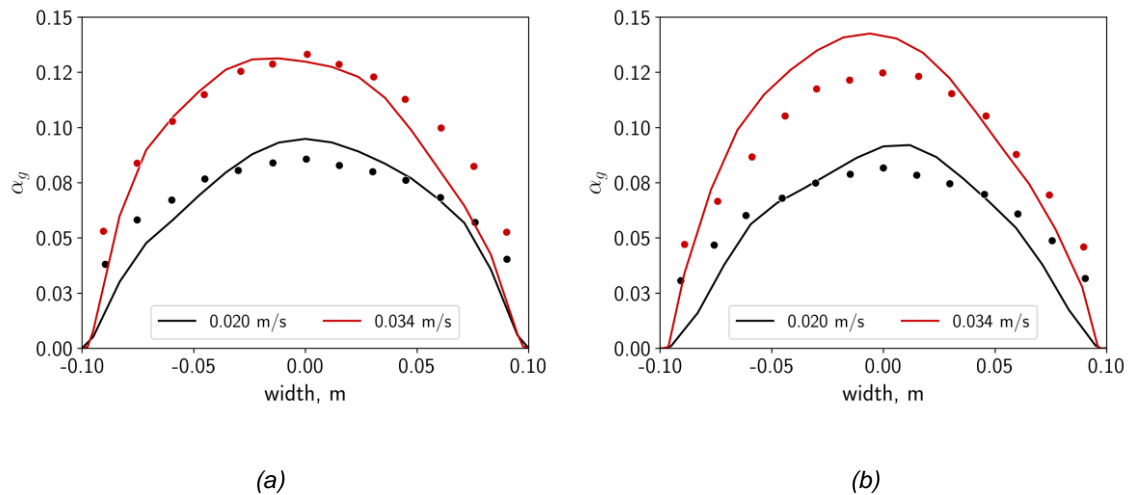
Figure 3: Local gas hold-up at height z/L = 3 at superficial gas velocity 0.02 and 0.034 m/s with 10% (a) and 20% (b) solid loading.
