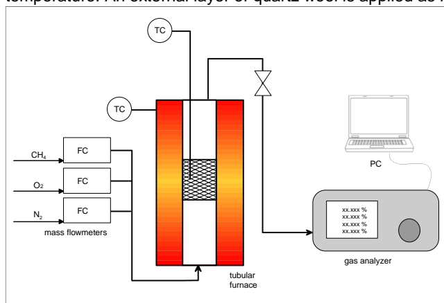
Figure 3: Schematic diagram of the experimental rig
