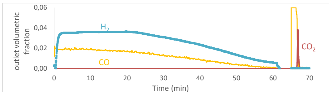
Figure 4: volumetric fraction of the off gases as a function of time during (1) the reductant in CH 4 10% (2) purge in N 2 , (3) oxidation in synthetic air ( y_{O_2}=0.21 )
