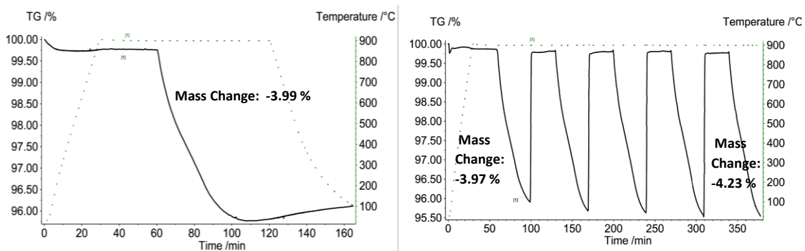
Figure4: thermogravimetric analysis of ceria, a) weight loss during a single reduction stage b) subsequent weight loss/gain in 4 cycles of reduction/oxidation
