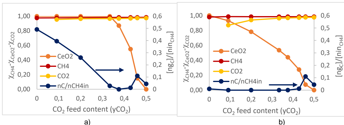
Figure 2: Effects of CO 2 extent on reactants conversion and carbon black formation in the feed stream with a [O]/[CH 4 ] ratio of a) 0.25 and b) 0.5. Data calculated at 910 °C and 1 atm from Aspen Plus process simulator.
