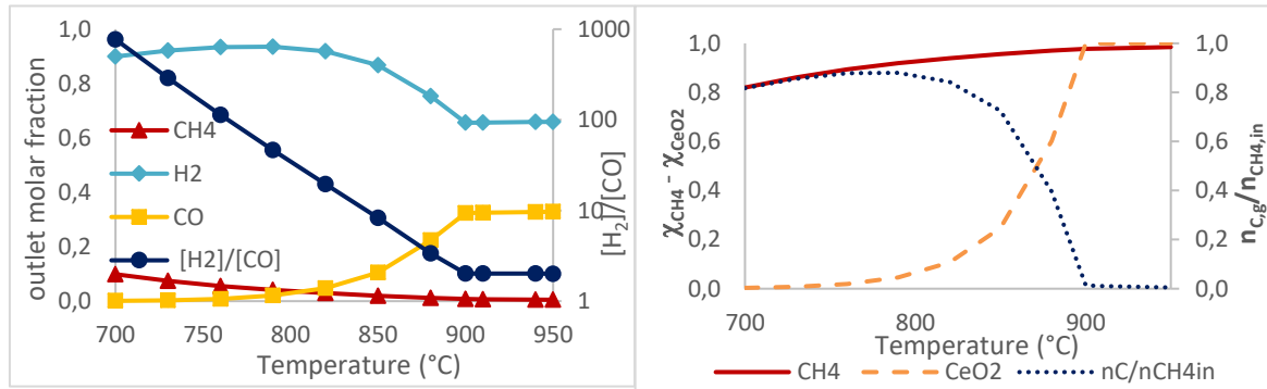
Figure 1: a) Reaction outlet composition of the gas phase at various process temperatures, using CeO 2 /CH 4 in stoichiometric ratio, calculated by process simulation analysis; b) effects on conversion and carbon extent in the range 700-950 °C
