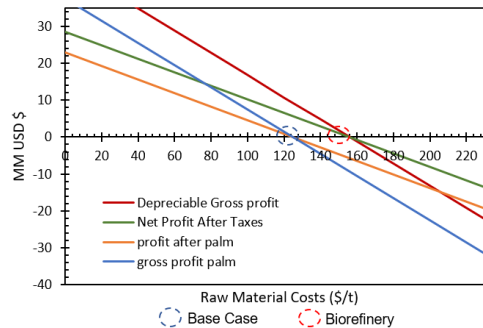
Figure 4: Effect of raw material cost on profitability for palm oil production chain and palm-based biorefinery
