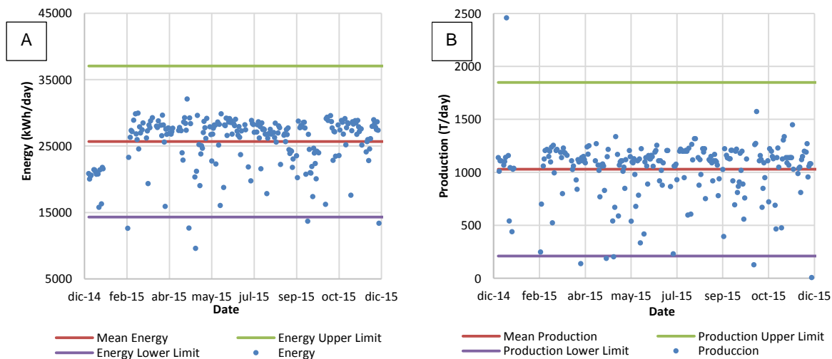
Figure 2. Boundary control charts a) Energy Consumption, b) Equivalent production of fertilizers.
