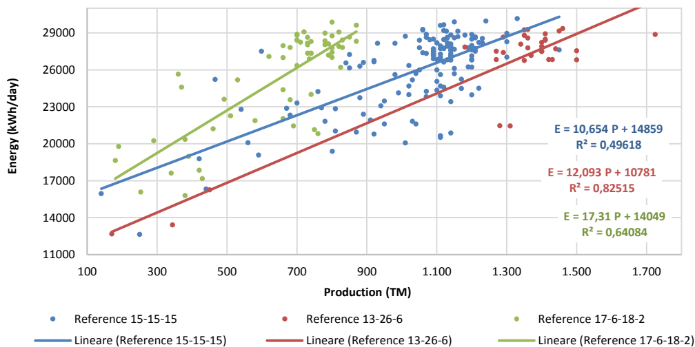
Figure 1. Base lines for energy consumption for three different produced fertilizers.
