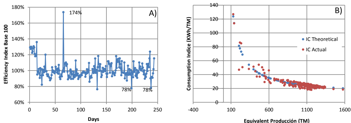
Figure 3. Energy Performance Indicators for the fertilizer plant. a) Index of base 100 efficiency, b) Index of energy consumption.
