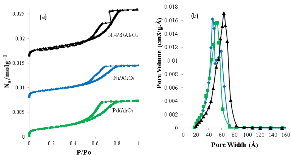
Figure 1: (a) Adsorption/desorption isotherms (b) and pore size distribution of calcined catalysts. The symbol represents: (◆) Ni/Al 2 O 3 ; (■) Pd/Al 2 O 3 and (▲) Ni-Pd/Al 2 O 3 .
