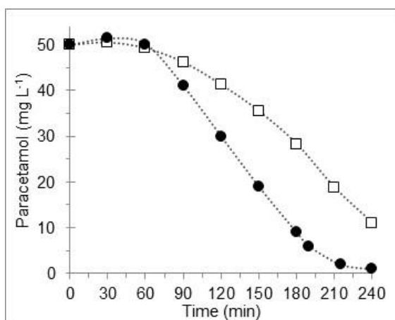
Figure 5: Removal of Paracetamol during UV/ \text{H}_2\text{O}_2 treatment with in situ electrogenerated hydrogen peroxide. Condition: 50 \text{mg L}^{-1} Paracetamol, 0.05 M \text{Na}_2\text{SO}_4 , volume 100 mL, current density 100 \text{A m}^{-2} , new cathode (●), aged cathode (□).
