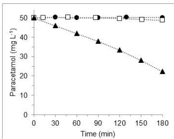
Figure 1: Removal of 50 mg L -1 Paracetamol by using 350 mg L -1 H 2 O 2 (●), UV irradiation (□) and combined UV/H 2 O 2 (▲) treatments.
