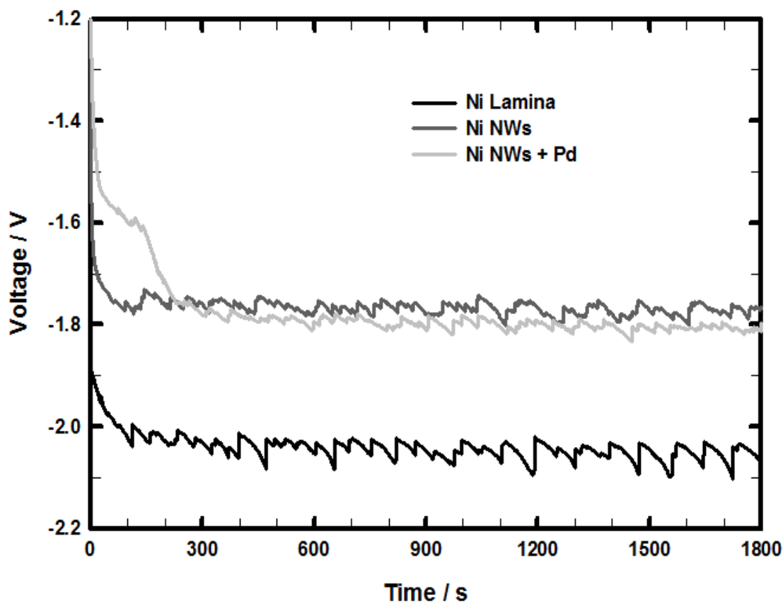
Figure 5: electrode voltage as a function of time at 0.05 \text{ A cm}^{-2} for alkaline water electrolyzer assembled with different cathodes and Ni Lamina as anode in 30% w/w KOH solution at room temperature.
