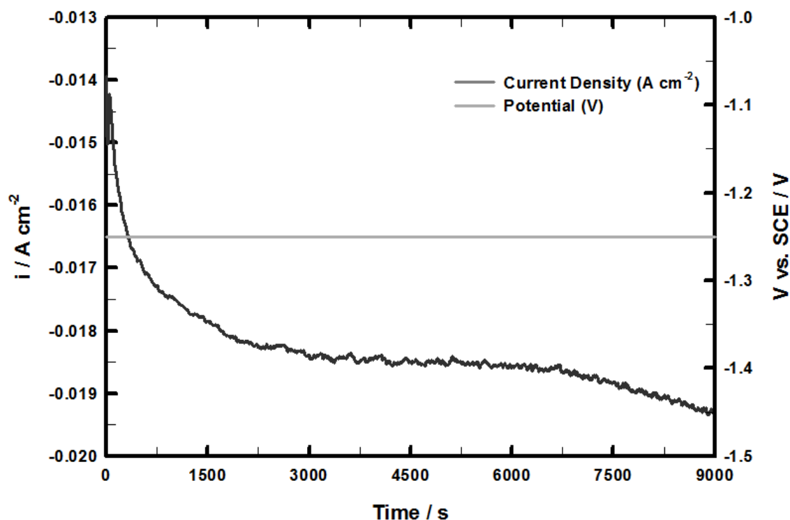
Figure 1: Ni layer electrodeposition potential and current density vs. time curves.
