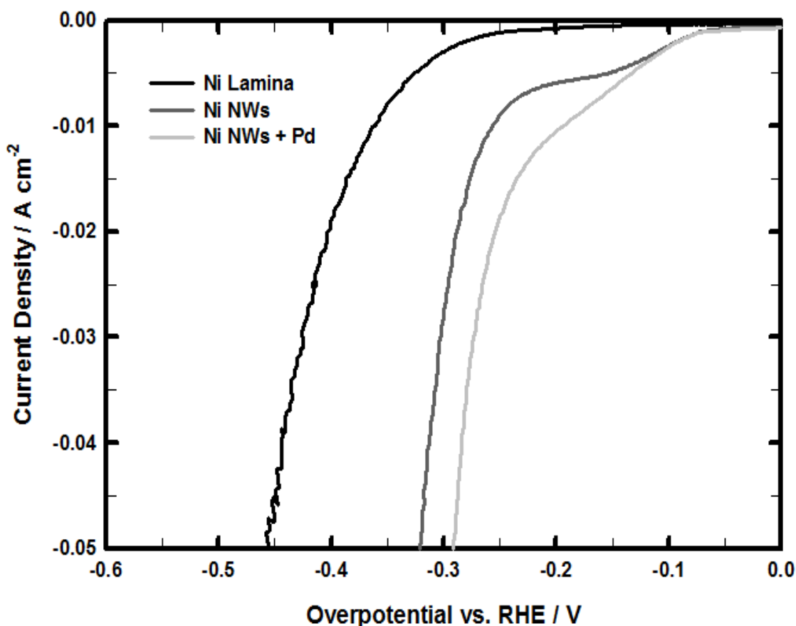
Figure 4: Quasi steady state polarization curves (scan rate 0.167 mV/s) measured for different electrodes in 30% w/w KOH solution at room temperature.
