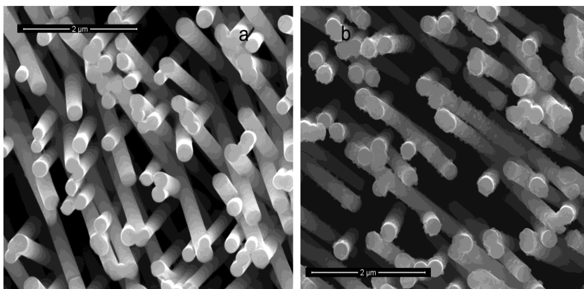
Figure 2: SEM images of nanostructured electrodes; a) Ni nanowires, b) Ni nanowires with Pd nanoparticles.
