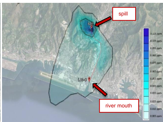
Figure 4: Isopleth airborne concentration (0- 15 hours).
