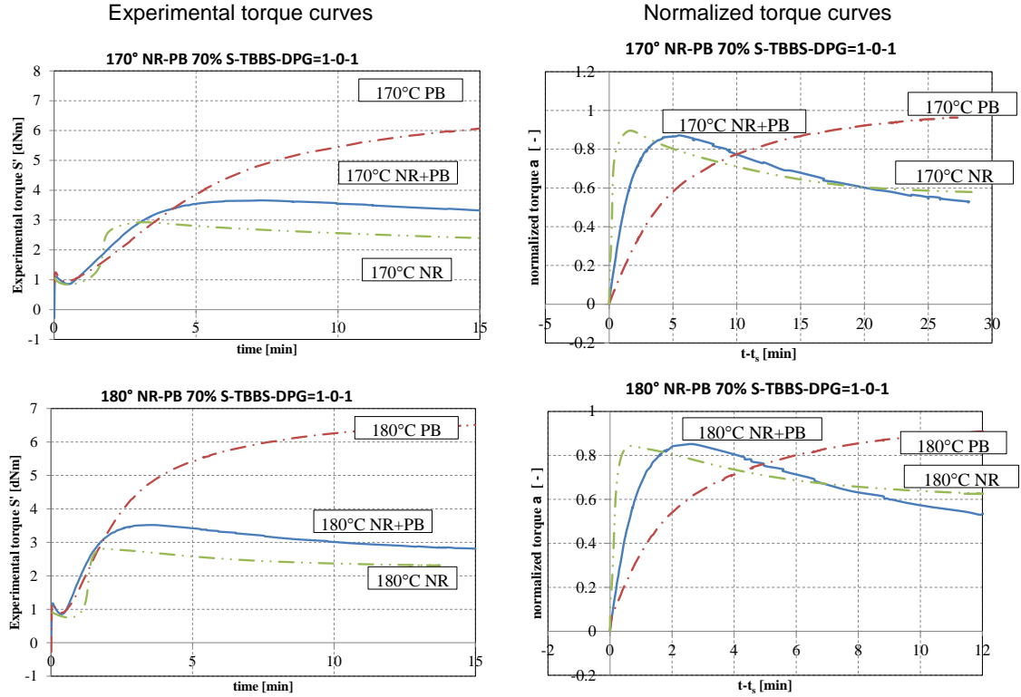
Figure 2: Experimental torque curves (left) and normalized curves (right) for natural rubber (NR), polybutadiene (PB) and 70% NR-30% PB blends at 170°C and 180°C Concentration of sulphur S and TBBS-DPG accelerants equal to 1-0-1.
