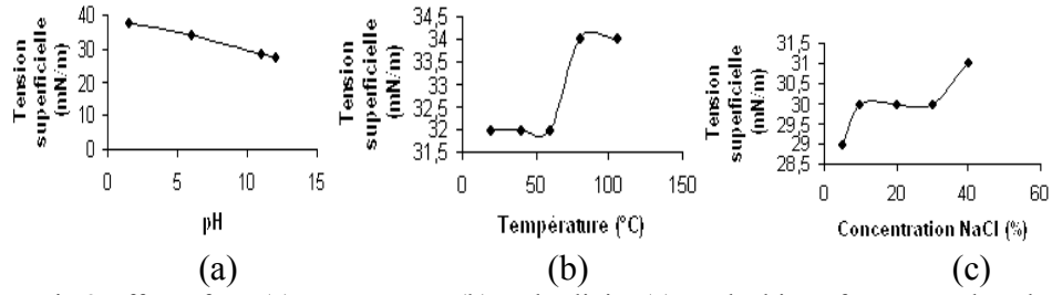
Fig.2.Effect of pH (a), temperature (b) and salinity (c) on the biosurfactant produced during P. fluorescens growth.
