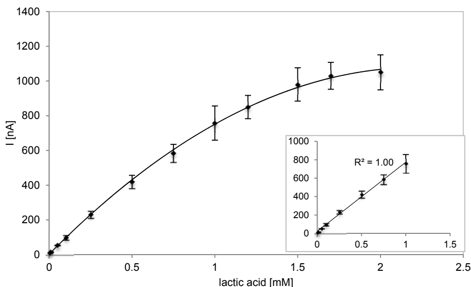
Figure 2: LOX biosensor calibration curves as average of five different biosensors. Inset: linear range of a LOX biosensors.
