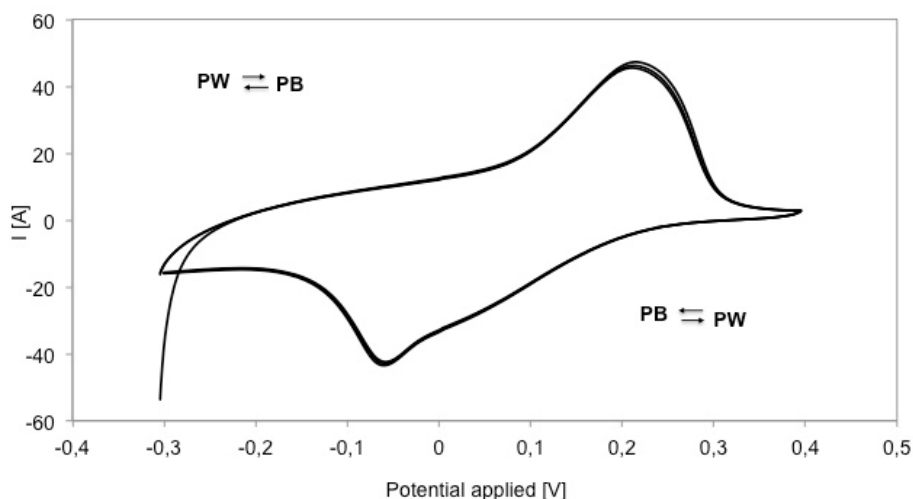
Figure 1: Cyclic voltammetry from -0.3 V to 0.4 V vs. Ag/AgCl of PB-modified screen-printed carbon electrode in 0.05 M phosphate buffer, 0.1 M KCl, pH 6.8.
