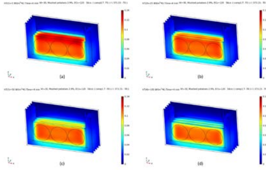
Figure 2. Slice plot of temperature after 4min. APG = 3 V/cm, MP29, (a) 5 W/(m 2 K), (b) 25 W/(m 2 K), (c) 50 W/(m 2 K) and (d) 100 W/(m 2 K)
