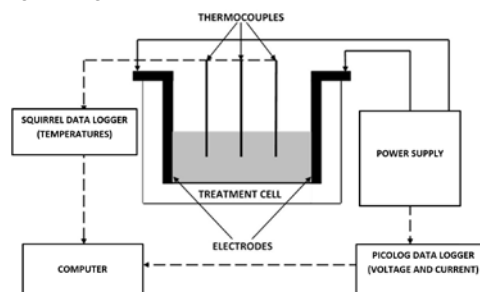
Figure 1. MEF heating equipment
