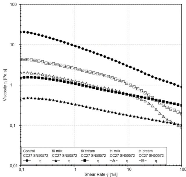
Figure 1: Flow curves of samples: apparent viscosity (Pa*s) as function of shear rate ( s^{-1} ) at 25°C obtained for the control (black circle), after dilution(t0) with cream (black squared) and milk (black triangles), and sprayed milk (white triangles) and cream (white squared) (t1) batter.
