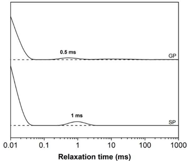
Figure 2: Continuous distribution of spin-spin relaxation times ( T_{1A} , obtained from CPMG experiment) of pure starch and pure gluten samples without any water addition
