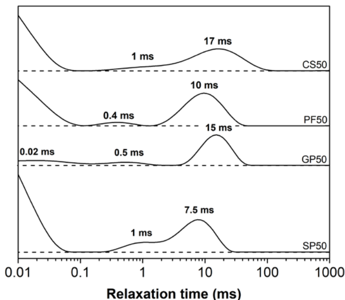
Figure 1: Continuous distribution of spin-spin relaxation times ( T_{1A} , obtained from CPMG experiment) of gluten-water and starch-water mixtures, commercial semolina dough, and pastry flour dough, at a water content of 50%
