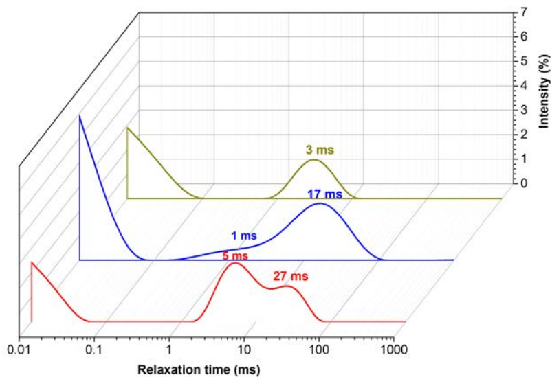
Figure 3: Continuous distribution of spin-spin relaxation times ( T_{1A} , obtained from CPMG experiment) of CS30 (dark yellow line), CS50 (blue line), and CS70 (red line)
