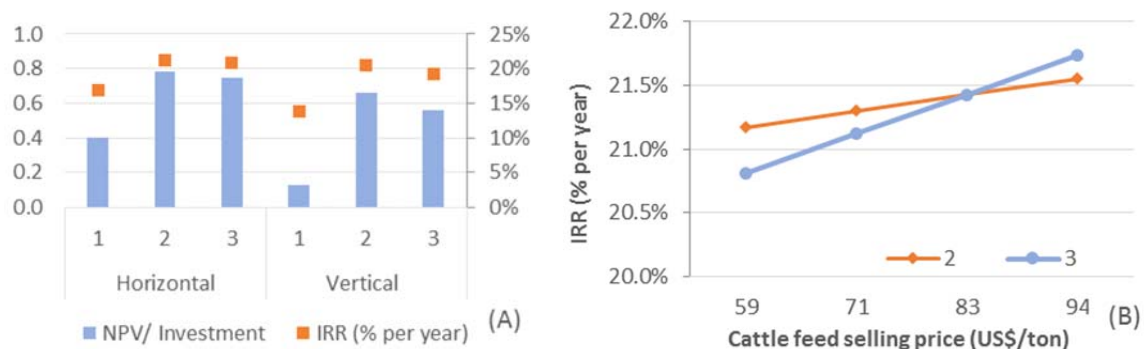
Figure 3: Techno-economic results: (A) NPV/investment and IRR for evaluated scenarios; (B) Sensitivity analysis of cattle feed price in the IRR of the sugarcane mill (horizontal approach).
