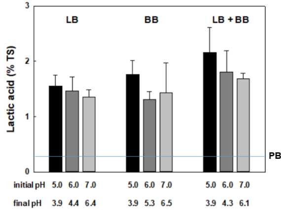
Figure 1: Lactic Acid production (% TS) for different pH tested values and employed bacteria communities.
