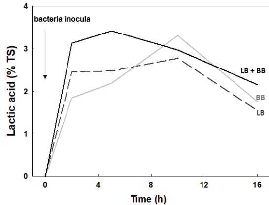
Figure 2: Lactic acid time evolution (% TS) for different employed bacterial communities in the fermentation process.
