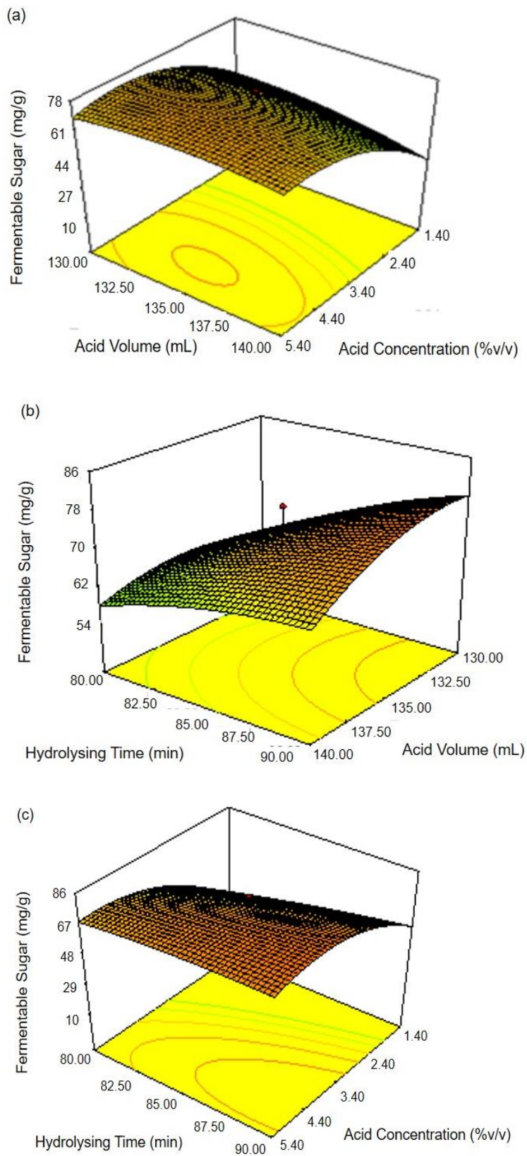
Figure 3: 3-D graph of the effect of (a) acid concentration ( x_1 ) and acid volume ( x_2 ), (b) acid volume ( x_2 ) and hydrolysing time ( x_3 ), and (c) acid concentration ( x_1 ) and hydrolysing time ( x_3 ) on the yield of fermentable sugar
