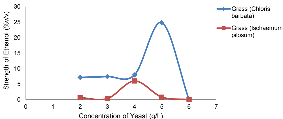
Figure 4: Strengths of ethanol obtained at different dosage of yeast in fermentation
