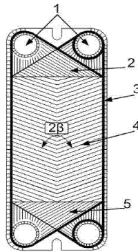
Figure 1: Schematic drawing of PHE plate: 1 – heat carrier inlet and outlet; 2,5 – zones for flow distribution; 3 – rubber gasket; 4 – the main corrugated field.
