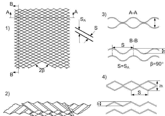
Figure 2: Different corrugation forms 1, 2 – the intersection of the adjacent plates; 3 – channel cross sections for the sinusoidal form of corrugations; 4 – channel cross sections for the triangular form of corrugations.
