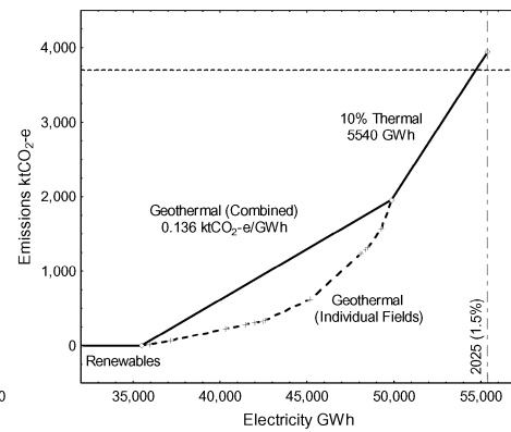
Figure 4. Geothermal section breakdown by individual fields.
