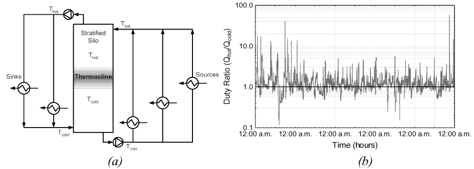
Figure 1. Industrial heating recovery loop (a) with simultaneous storage of hot and cold water in a stratified silo for smoothing variable heating and cooling duties (b).
