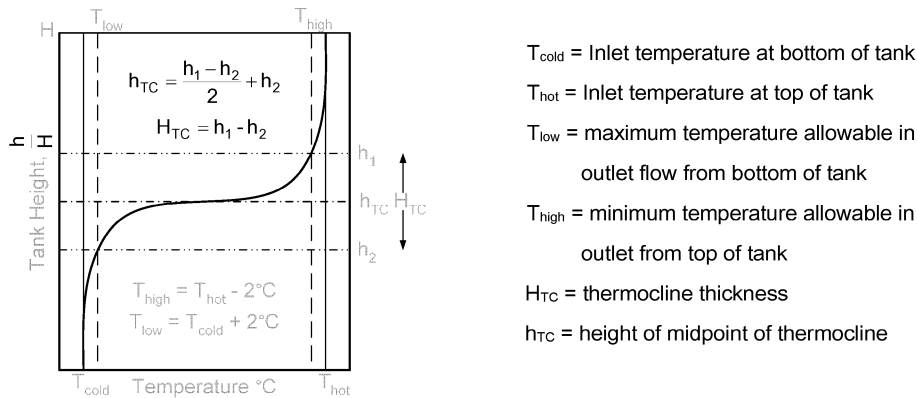
Figure 3. Illustration of variables used to describe a thermocline in a stratified tank.
