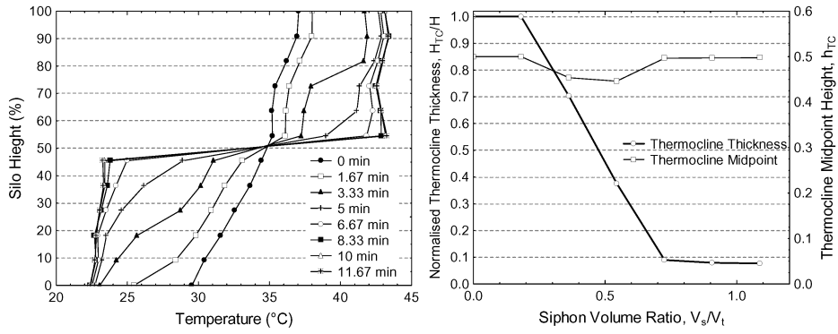
Figure 5. Interface re-establishment with siphoning from 50% height, perspex tank, siphon rate 0.7LPM.
