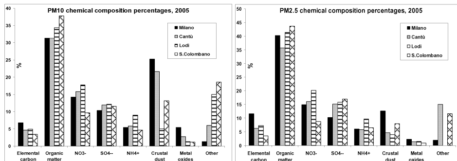
Figure 4.1: PM 10 chemical composition percentages. Parfil project, 2005
