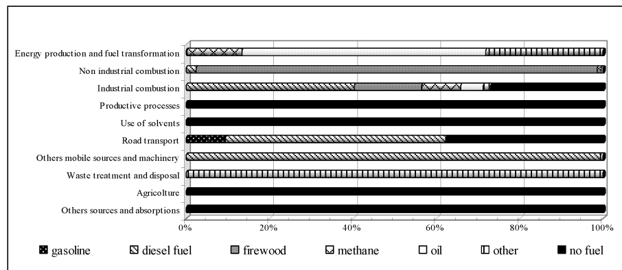
Figure 3.1 Lombardy region 2005 PM_{10} emissions (t/year), distinguished in macro sector and fuel.
