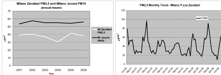
Figure 2.4: Annual trend for Piazza Zavattari PM_{2,5} and Juvara PM_{10} stations, Milan.
