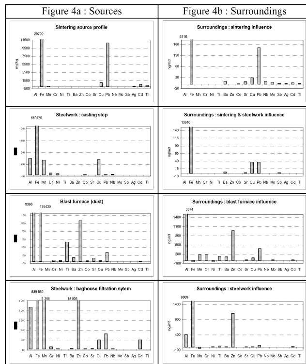
Figure 4: Profile comparison between source and environment
