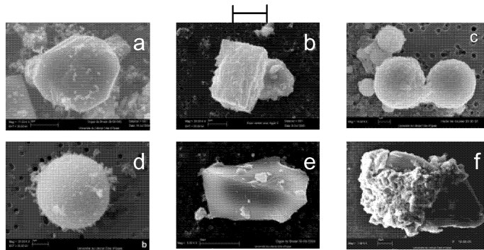
a) angular shape of Fe ores (scale:4 \mu\text{m} ); b) K and Cl rich particles (scale:5 \mu\text{m} ); c) and d) Spherical iron oxide (scale:3 \mu\text{m} ); e) graphite flake (scale:10 \mu\text{m} ); f) graphite flake (scale:25 \mu\text{m} ) covered by Fe-Ca-Si aggregates (left side)
