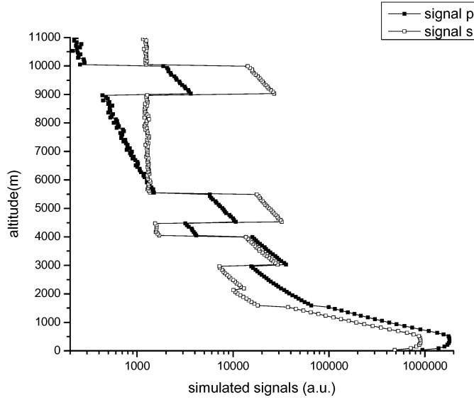
Fig.1 Simulated signals for parallel and orthogonal directions of polarization. The parallel one is indicated by the full square and the orthogonal one by the empty square.
