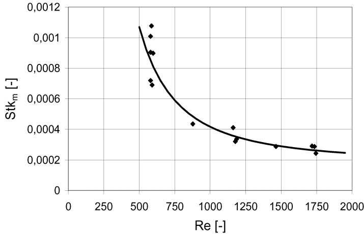
Fig.4 – Dependance of Stk_m on Re
