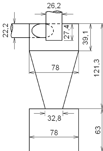
Fig. 1 – Main dimensions of cyclone
