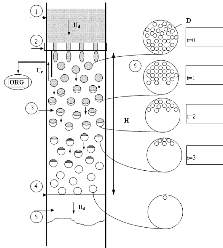
Figure 1 - Principle of operation of the MDIF®. Source: Paulo et al. (1994).
