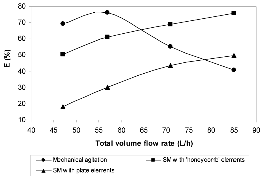
Figure 2 - Total efficiency of separation as function of total volume flow rate.
