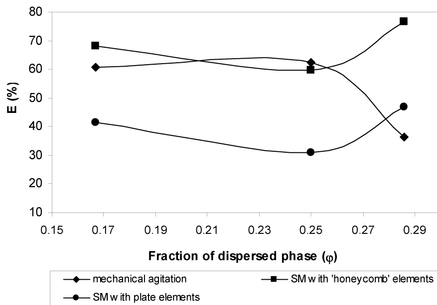
Figure 3 – Total efficiency of separation as function of fraction of dispersed phase.
