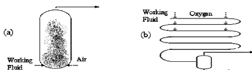
Figure 1: H 2 O 2 reactor unit process (a) before and (b) after process intensification
