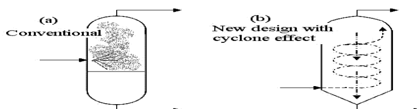
Figure 2: H 2 O 2 phase separator details with (a) high and (b) low of mist formation
