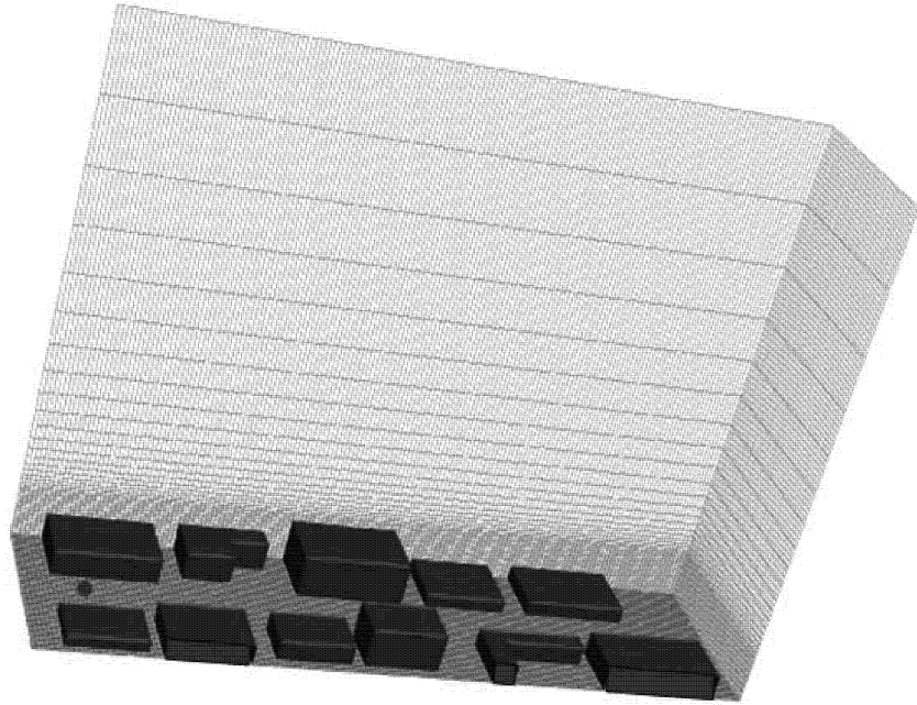
Fig. 2: Computational grid
