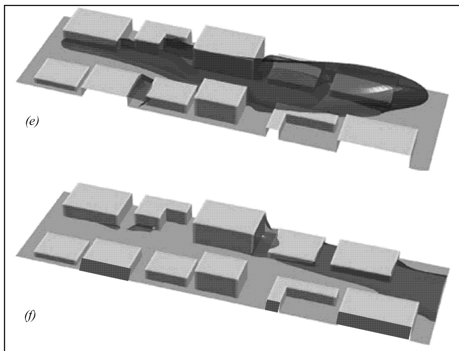
Fig. 5: Constant Chlorine concentration iso-surfaces at 1 (a), 10 (b), 30 (c), 60 (d), 180 (e) and 300 (f) seconds after the release
