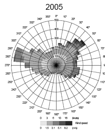
Fig. 2 Wind rose of the Ferrara territory (data from Regional Agency for Environment Protection)
