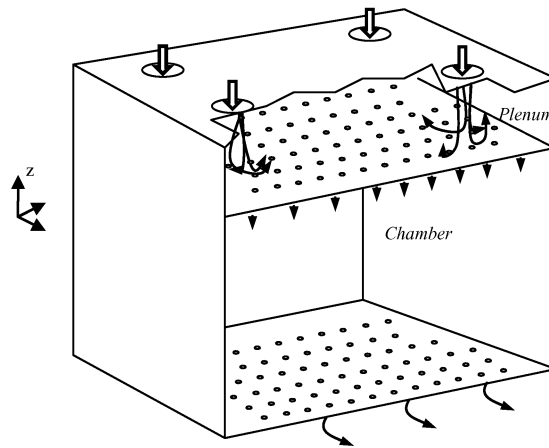
Figure 1: Sketch of the proposed exposure chamber.
