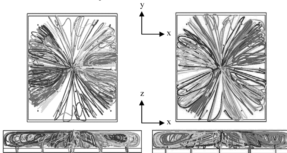
Figure 4: Particle trajectories into the plenum: 1 \mu\text{m} (left) and 10 \mu\text{m} (right) particles.
