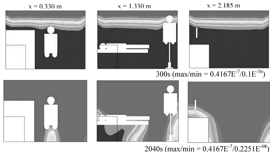
Figure 5: Aerosol concentration fields at three different locations within the chamber.
