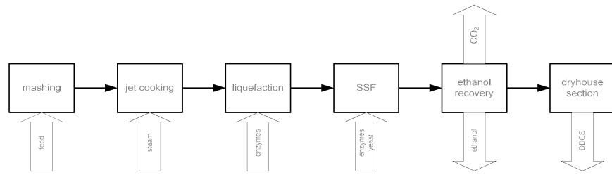
Figure 1. Process block diagram for the dry milling process.
