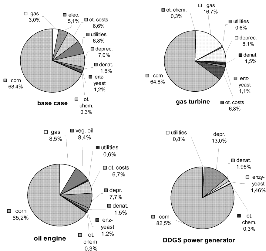
Figure 3. Costs allocation for the four different process cases.
