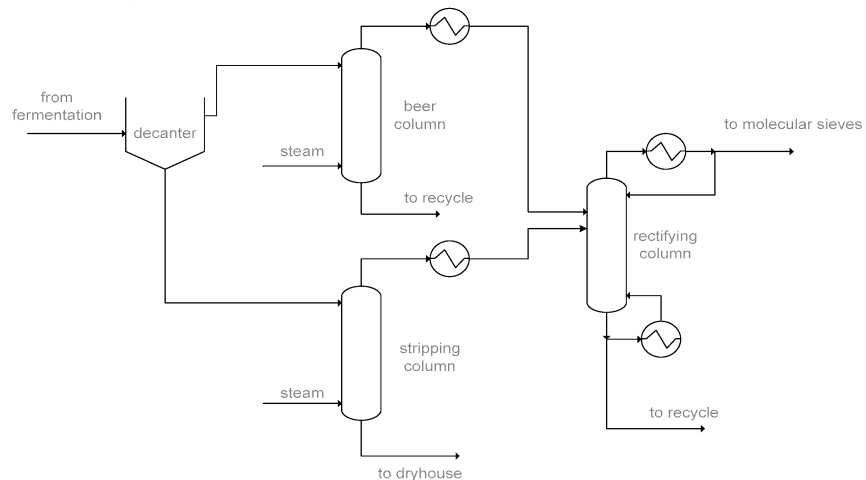
Figure 2. Process flowsheet of the ethanol recovery section in the dry milling process.
