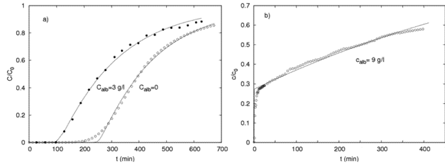
Fig. 2 Typical tryptophan and bilirubin breakthrough curves on activated carbon and anionic resin, respectively. Line: fitted mode, circles: experimental data..
