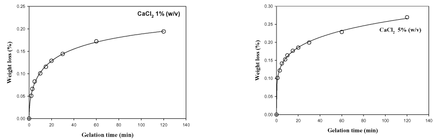
Figure 4 - Weight loss versus gelation time for a solution containing 2% (w/v) of alginate mixed with solution containing different concentrations \text{CaCl}_2 .
