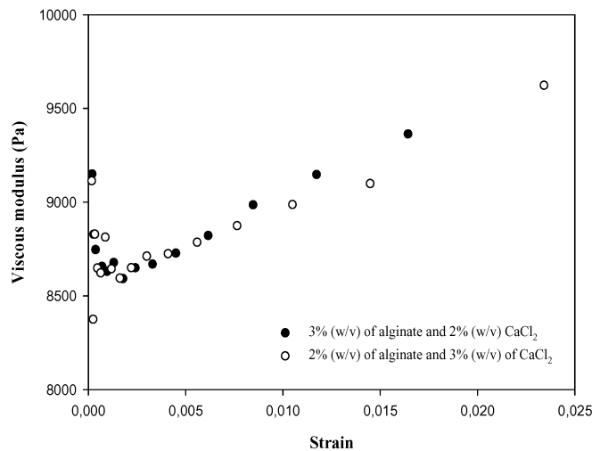
Figure 6 – Viscous modulus versus strain for two different alginate gels.
