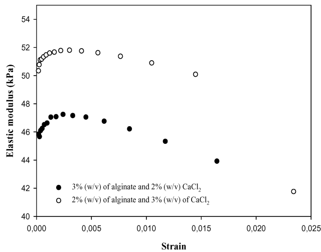
Figure 5 – Elastic modulus versus strain for two different alginate gels.
