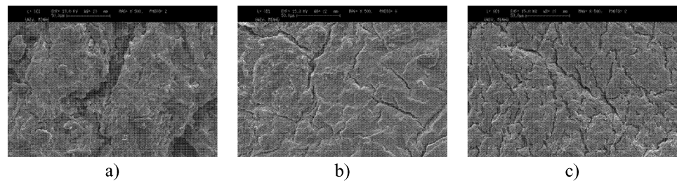
Figure 7 – SEM for gels containing 2% alginate and 1% \text{CaCl}_2 (a), 3% alginate and 1% \text{CaCl}_2 (b) and 2% alginate and 2% \text{CaCl}_2 (c).
