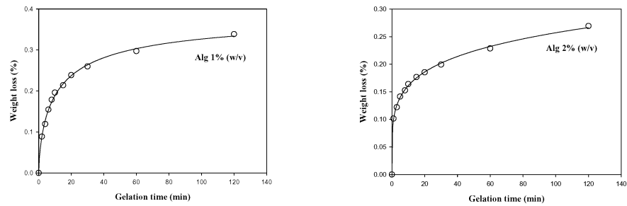
Figure 3 - Weight loss vs gelation time for two solutions containing different concentrations of alginate mixed with a solution of 5%(w/v) of \text{CaCl}_2 .
