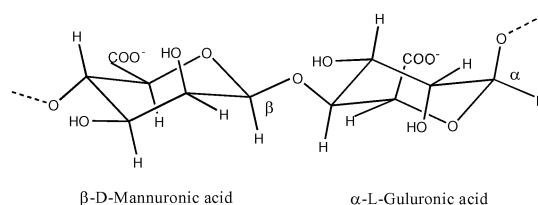
Figure 2 - Structure of an alginate showing a linkage between the M and G acids.
