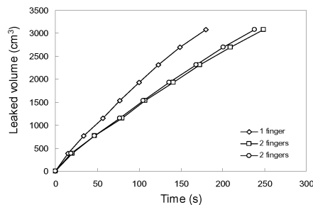
Figure 4. Leakage tests using a rectangular hole ( 6.00 \times 1.18 \text{ cm}^2 ) with a wall thickness of 0.8 cm and no grooves.
