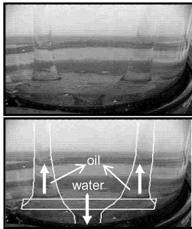
Figure 5. Formation of two similar oil fingers during leakage tests using a rectangular hole ( 4.60 \times 1.53 \text{ cm}^2 ) with a wall thickness of 0.8 \text{ cm} , no inclination and no grooves.
