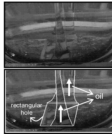
Figure 6. Formation of two different oil fingers during leakage tests using a rectangular hole ( 6.14 \times 2.05 \text{ cm}^2 ) with a wall thickness of 1.2 \text{ cm} , no inclination and no grooves.
