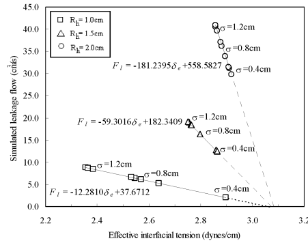
Figure 8. Leakage obtained from the phenomenological model as a function of the effective interfacial tension, considering three different hole radius.
