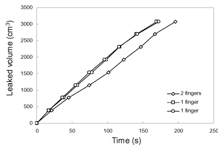
Figure 3. Leakage tests using a rectangular hole ( 4.60 \times 1.53 \text{ cm}^2 ) with a wall thickness of 0.8 cm and no grooves.
