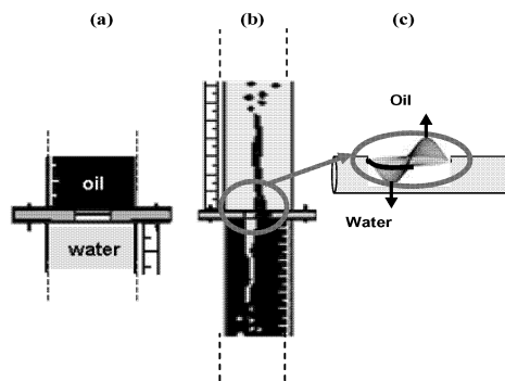
Figure 1. Detailed scheme of the experimental apparatus: a) Initial condition with a plane interface; b) Perturbed interface after a rotation of 180^\circ of the apparatus; c) real horizontal situation simulated with the experiments.
