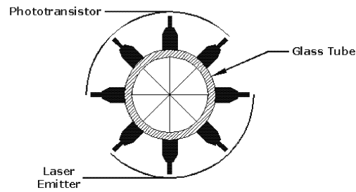
Figure 2. The multipoint sensor scheme.
