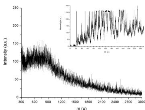
Figure 3. Reflectron LDI-MS spectrum of fraction 2 at 90% of the laser power. In the inset zoom in the low MW region.
