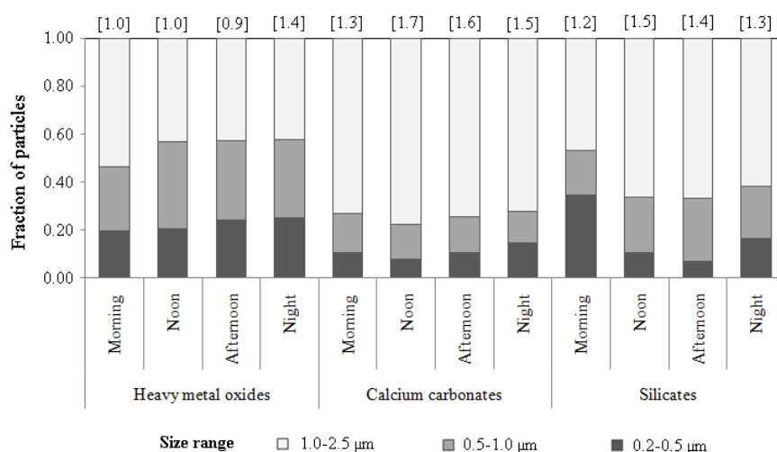
Figure 1. Fraction of particles in the 0.2-0.5 µm (dark grey), 0.5-1.0 µm (medium grey), 1.0-2.5 µm (light grey) in each cluster and period. Particle mean size placed in the top of the bar in brackets.
