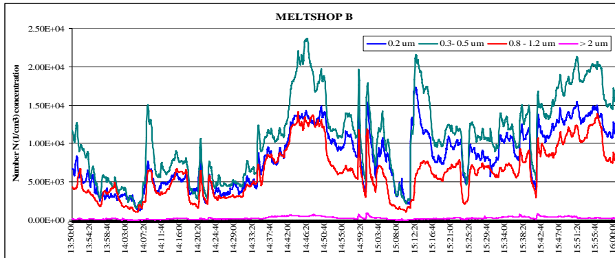
Figure 2 Number concentration dynamics: high-grade steel, low-quality scrap.
