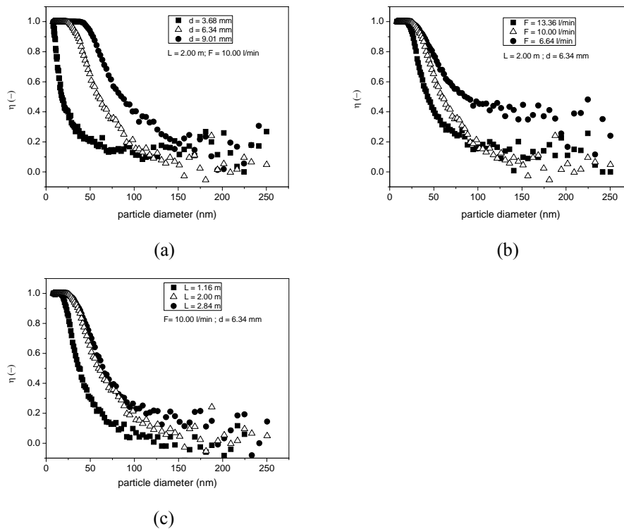
Figure 2 Experimental efficiency of nanoparticle deposition: (a) efficiency with diameter as variable; (b) efficiency with aerosol flow rate as variable and (c) efficiency with tube length as variable.
